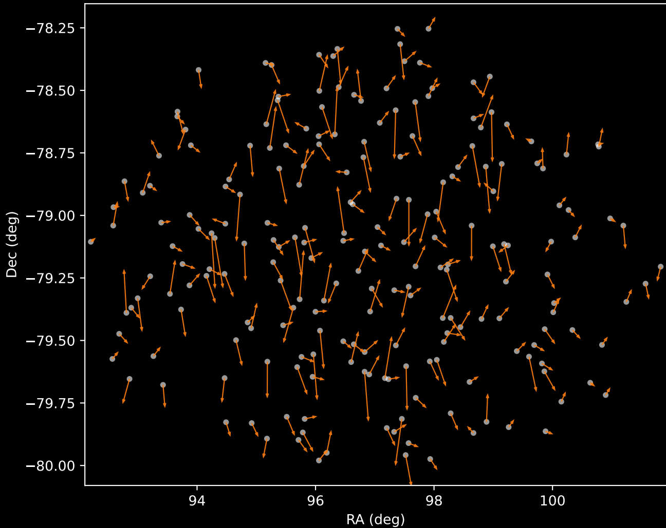
GALAH DR4 Cluster 2 Proper Motion Vectors (n=214)
