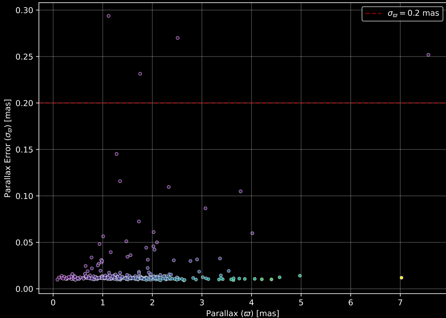
GALAH DR4 Field: [321] Parallax Quality (n= 279)
