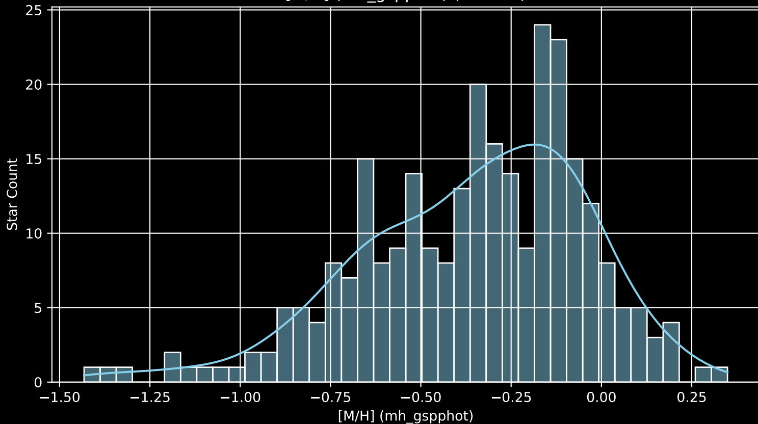
GALAH DR4 Field: [321] [M/H] (mh_gspphot) (n= 278)
