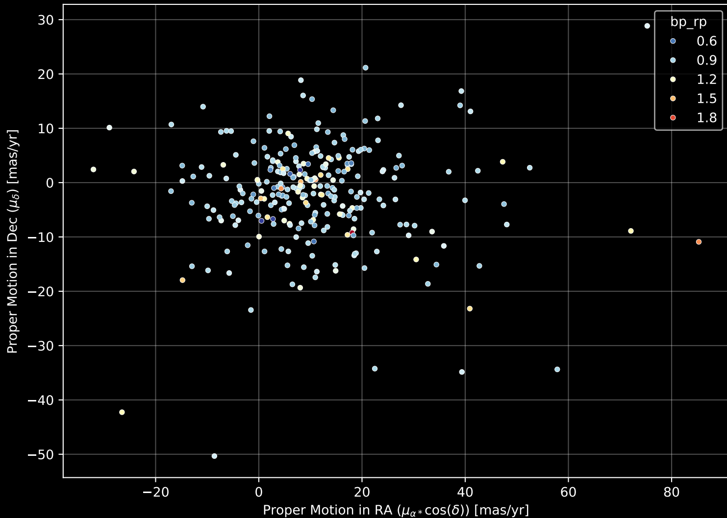
GALAH DR4 Field: [321] Proper Motion Diagram (n= 279)
