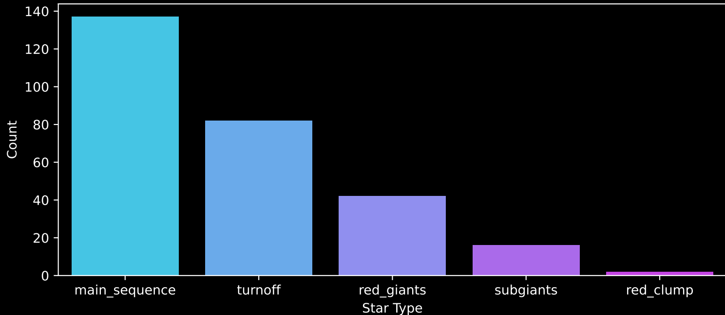
GALAH DR4 Field: [321] Count plot of Star Type
