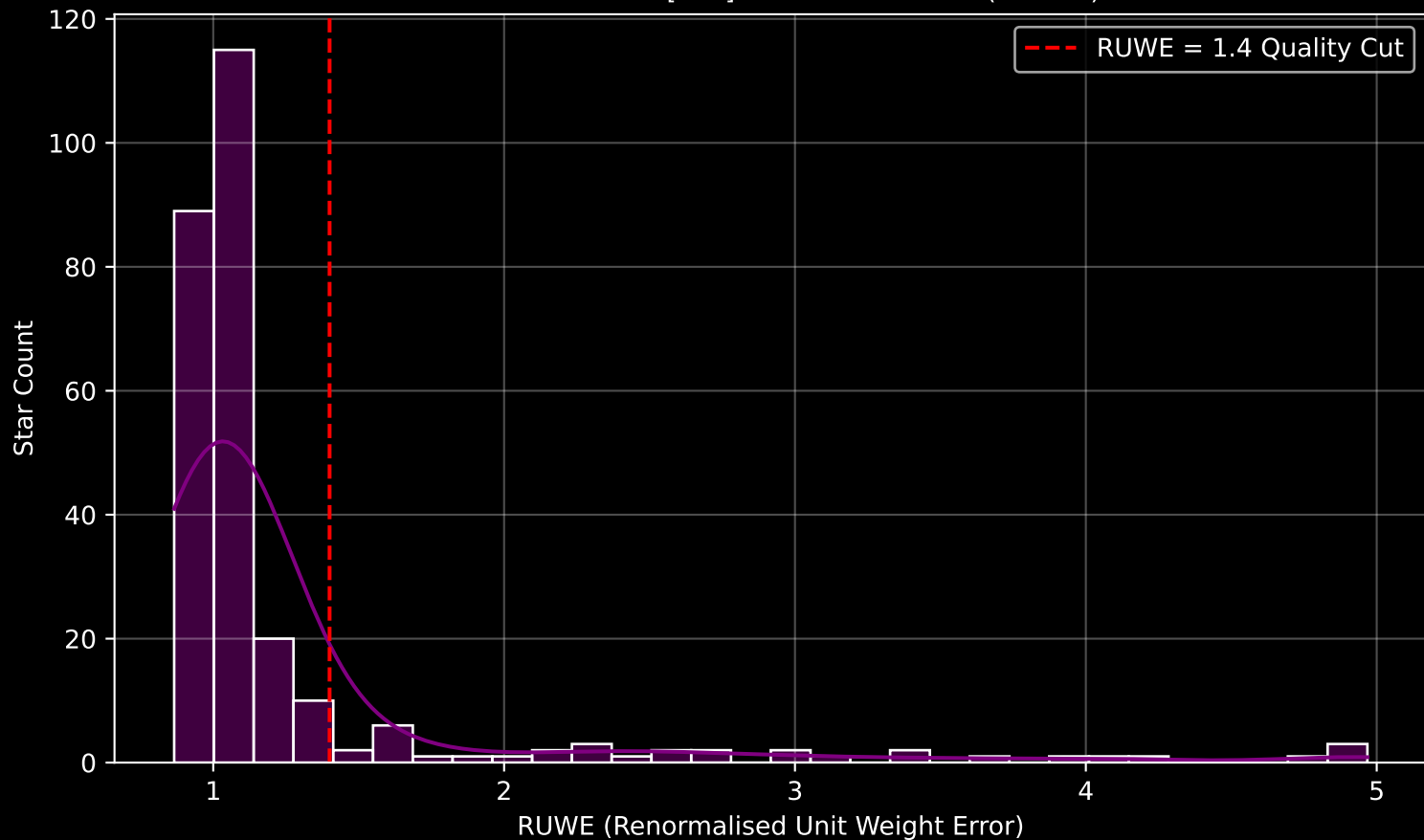
GALAH DR4 Field [321] RUWE Distribution (n= 268)
